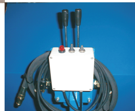
Manuel manøvreventil (standard)
